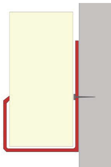
J-Channel
