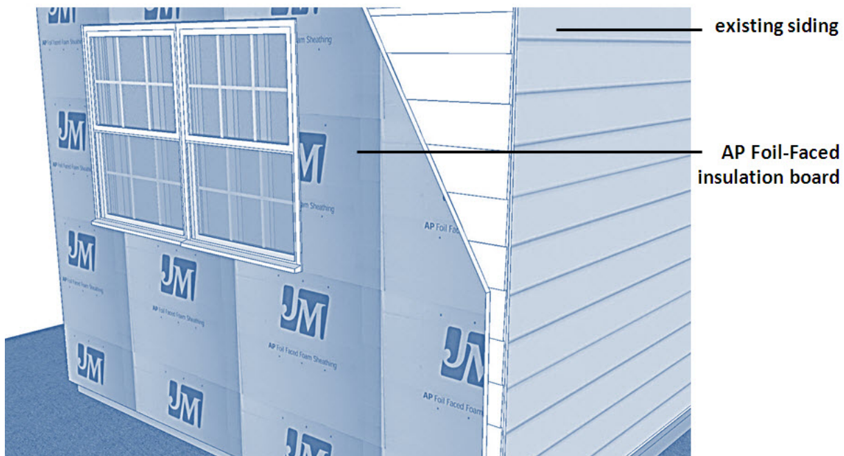
Figure 6. Existing Wall – AP™ Foil-Faced Insulation Over Siding
