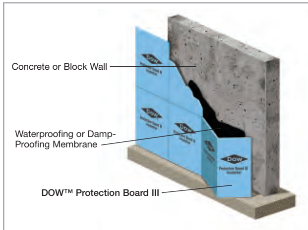
Fanfolded on 24" centers with plastic film on one side, DOW™ Protection Board III Insulation is durable yet easy to install and work with on the job site.
